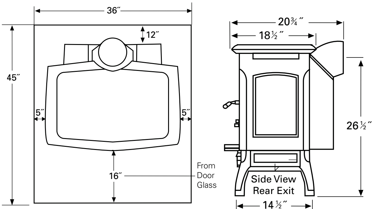
Minimum Hearthpad Dimensions Does not include the distance from the stove to the wall.
